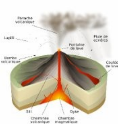
Eruption strombolienne
