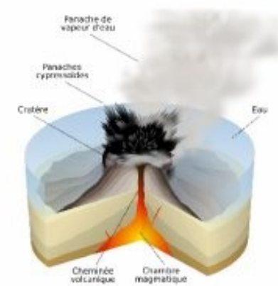
Eruption surtseyenne
